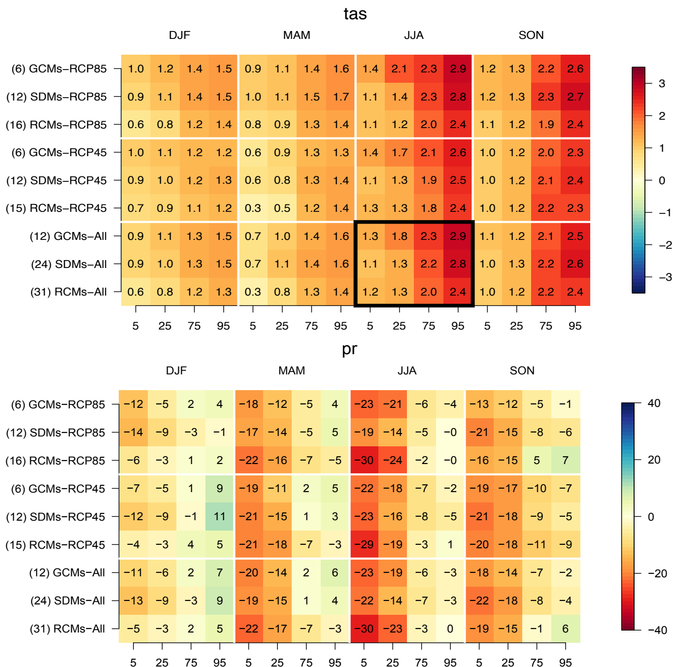
Figure 2: Projected changes for seasonal temperature (°C, top) and precipitation (% , bottom) by 2021- 2050, with respect to the average of the 1971-2000 period, on average for continental Spain and the Balearic Islands for two different forcing scenarios (RCP8.5, RCP4.5 and both “All”) considering the GCM, SDM, or RCM projections (in different rows for each scenario). In order to provide comprehensive information about the ensemble uncertainty in the climate change signal, different percentiles (5, 25, 75 and 95) are given for each case. The range 25-75 is the typical value used to characterize the ensemble spread, whereas 5th and 95th values characterize the extreme signals within the ensemble
