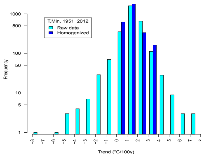
Figure 1: Trends of the Spanish minimum air temperatures before and after the homogenization of their series. Inhomogeneities in the raw observational data result in an abnormally high dispersion of the computed trends.
